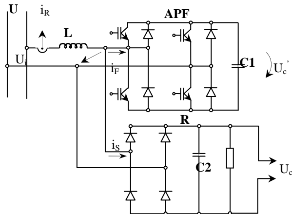
Fig.5. Simulation model.
