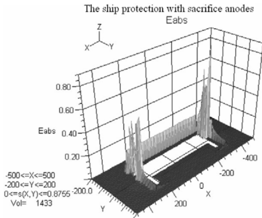
Fig. 15 The variation mode of electric field absolute value V_{seawater} \langle V_{sacrificeanode}
