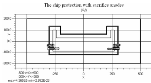
Fig. 16 The distribution of the current density vector V_{seawater} \langle V_{sacrificeanode} (V_{referenceanode} \cong V_{ship'shull})
