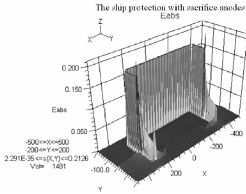
Fig. 3. The variation mode of electric field absolute value V_{seawater} \gg V_{ship'hull}
