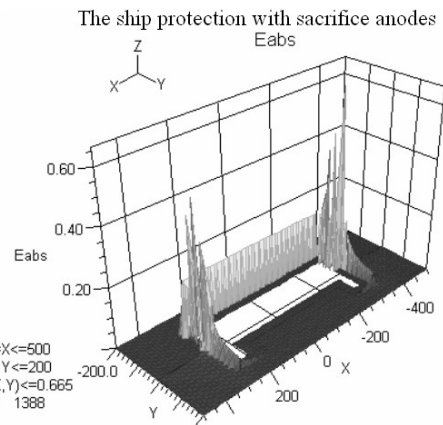
Fig. 12 The variation mode of electric field absolute value V_{seawater} \setminus V_{sacrificeanode}
