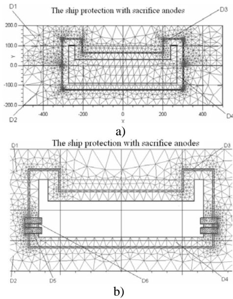
Fig. 1 The integration domain: a) in case there are no sacrificial anodes on the ship; b) when the ship is equipped with aluminium sacrificial anodes
