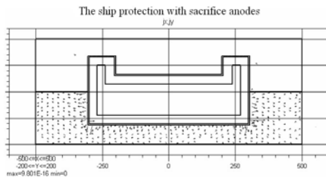
Fig. 4 The distribution of the current density vector V_{seawater} \gg V_{ship'hull} (without sacrifice anodes)
