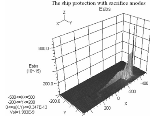
Fig. 6 The variation mode of electric field absolute value V_{seawater} = V_{ship'hull}
