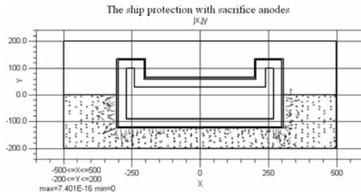
Fig. 7 The distribution of the current density vector V_{seawater} = V_{ship'hull} (without sacrifice anodes)
