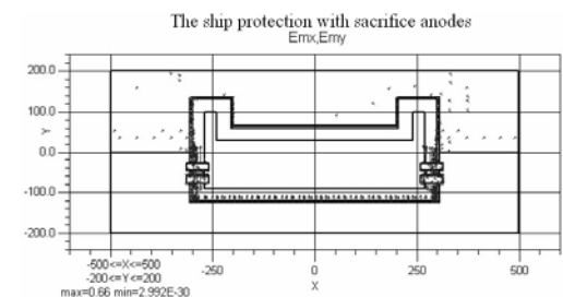
Fig. 14. The distribution of the electric field V_{seawater} \setminus V_{sacrificeanode} ( V_{referenceanode} \cong V_{ship'shull} )
