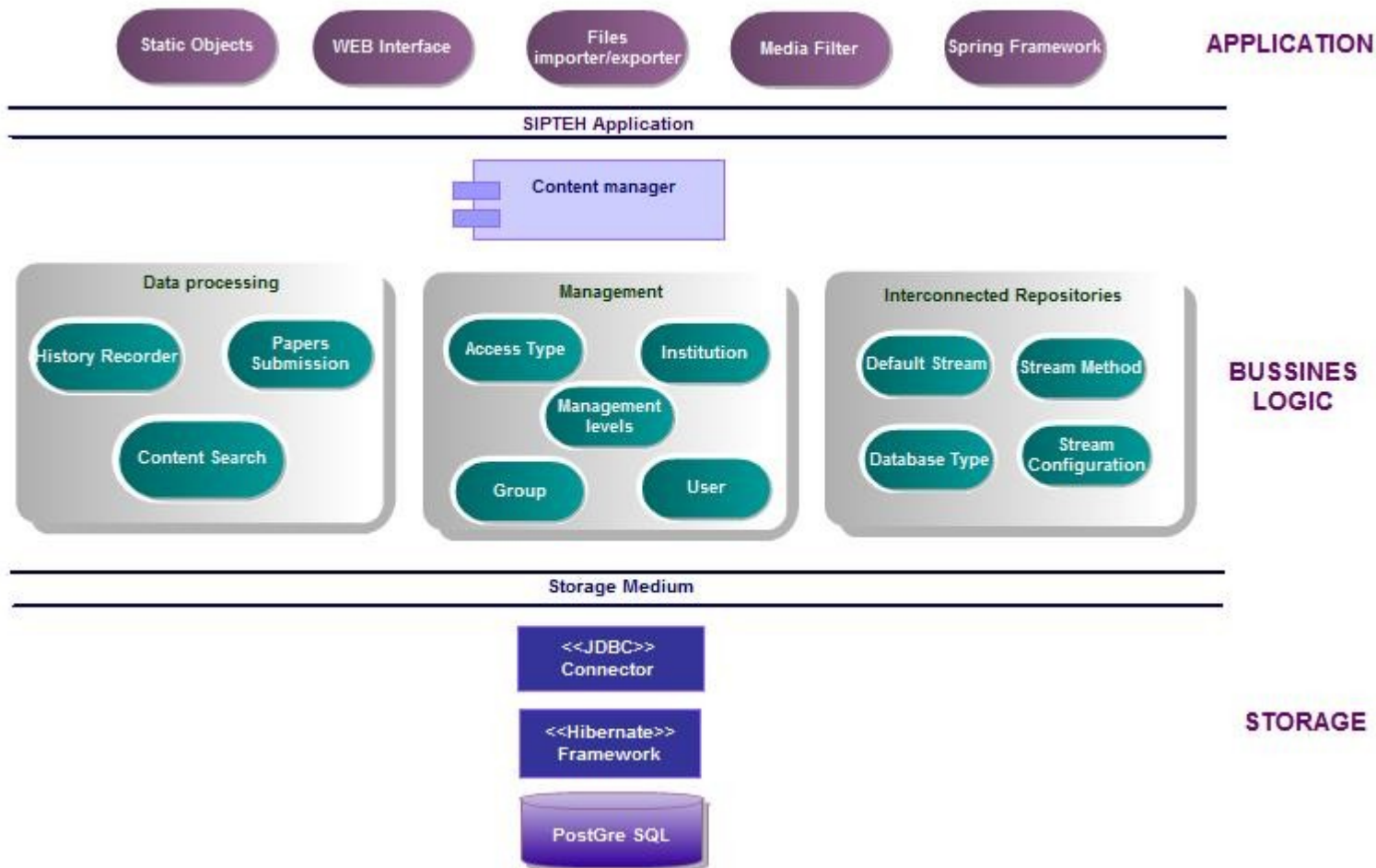
SIPTEH INTEGRATED SYSTEM ARCHITECTURE
